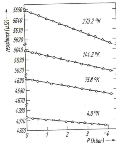
Fig. 2. Typical resistance versus pressure isotherms for the 25 at% Au-75 at% Ag alloy. \circ indicates increasing pressure and \triangle indicates decreasing pressure
